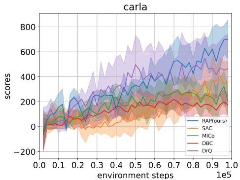
Figure 6: Training curves on CARLA.
